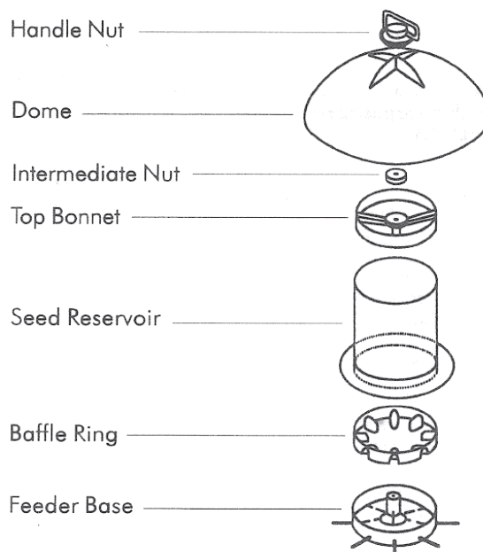
Carousel Feeder
